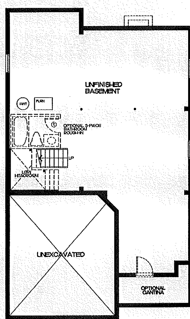
40-5 BASEMENT ELEVATION A GFA = 2510 SF
