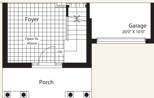
Ground Floor Elevation B
