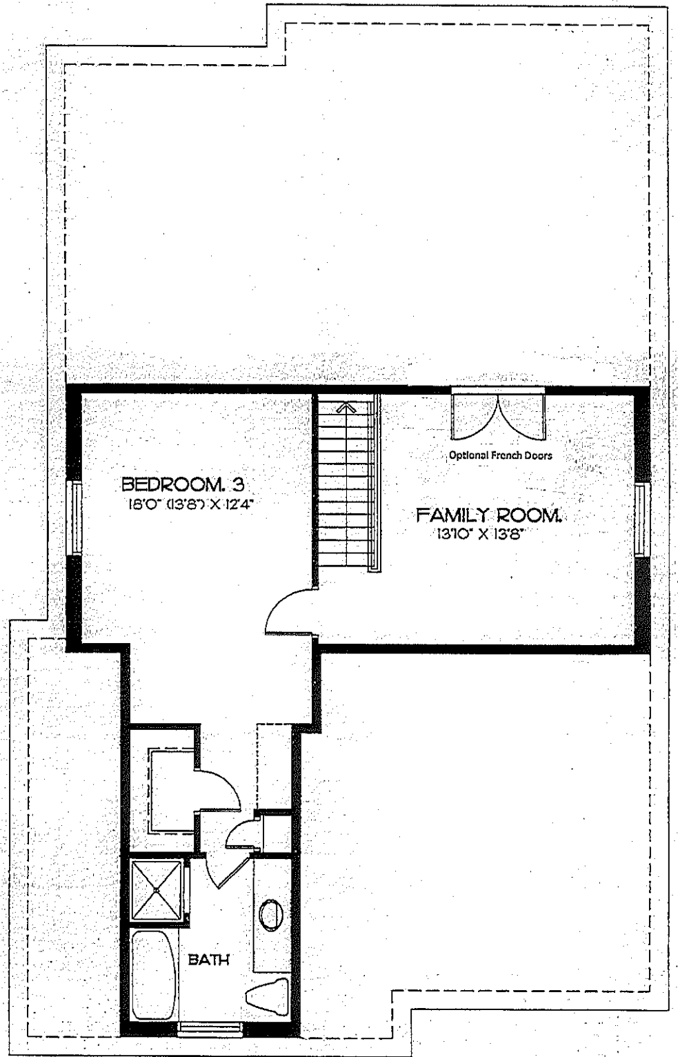
SECOND FLOOR
