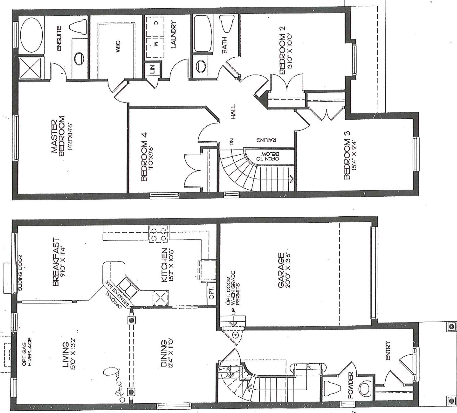
GROUND FLOOR ELEVATION 'A'
